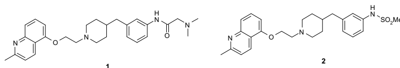
Figure 1. Examples of potent analogues from previous studies with basic and non-basic phenyl substituents.
