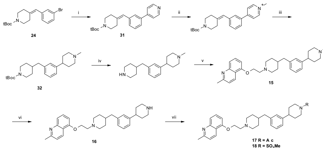
Scheme 3. Reagents and conditions: (i) 4-pyridyl boronic acid, Pd(Ph 3 ) 4 , Na 2 CO 3 , H 2 O/DME, reflux, 54%; (ii) MeI, DCM, rt, 95%; (iii) Pt 2 O, H 2 , EtOH, 50 °C, 88%; (iv) HCl, Et 2 O, rt, 100%; (v) 26 , K 2 CO 3 , DMF, 100 °C, 16 h, 40%; (vi) ClO 2 CCHClCH 3 , t Pr 2 NEt, 1,2-dichloroethane, reflux, 62%; (vii) for R = Ac; Ac 2 O, Pyr, DCM, rt, 61%; for R = SO 2 Me, MeSO 2 Cl, t Pr 2 NEt, NEt 3 , DCM, rt, 70%.
