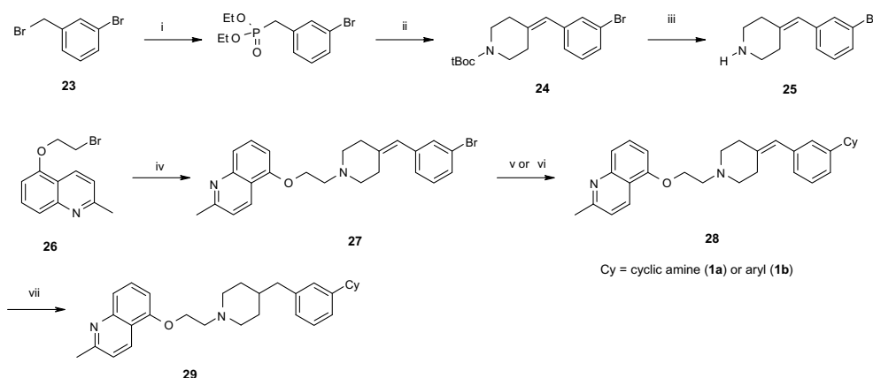
Scheme 1a (Buchwald) and 1b (Suzuki). Reagents and conditions: (i) P(OEt) 3 , toluene, reflux, 24 h, (85%); (ii) N -Boc-piperid-4-one, NaH, THF, rt, 4 h (89%); (iii) 1 M HCl in Et 2 O, rt, 72 h (57%); (iv) 25 , K 2 CO 3 , DMF, 100 °C, 16 h, 87%; (v) amine, Pd(OAc) 2 , BINAP, Cs 2 CO 3 , 1,4-dioxane, reflux (39–100%); (vi) CyB(OH) 2 , PPh 3 , 2 M aq K 2 CO 3 , Pd(OAc) 2 , reflux, 1,2-DME; (vii) 10% Pd on C, H 2 , EtOH, rt, 24 h, (9–100%).
