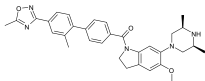
Figure 2. Structure of SB-616234, a selective 5-HT 1B receptor antagonist.
