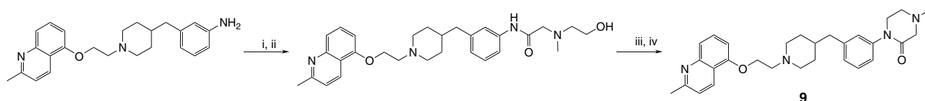
Scheme 2. Reagents and conditions: (i) chloroacetylchloride, Et 3 N, rt, DCM; (ii) MeNCH 2 CH 2 OH, t Pr 2 NEt, NaI, rt, i PrOH; (iii) ClSO 2 Me, Pyr, rt; (iv) NaH, DMF, rt to 50 °C, 22% over entire sequence.
